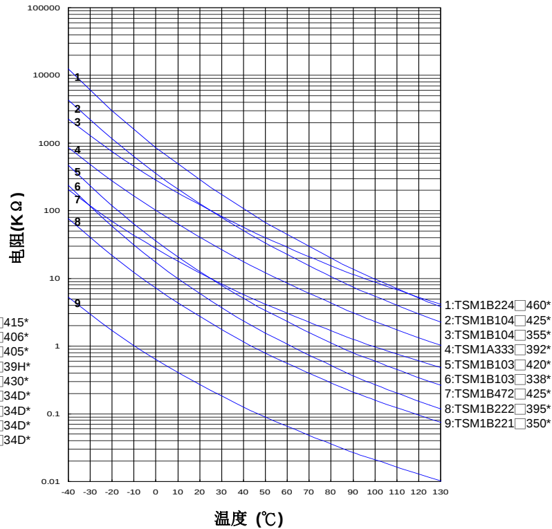
TSM1B221□350* ~ TSM1B224□460*
