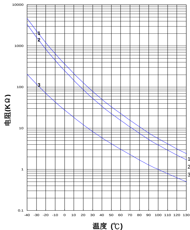
TSMAB103□338* ~ TSMAB104□425*
