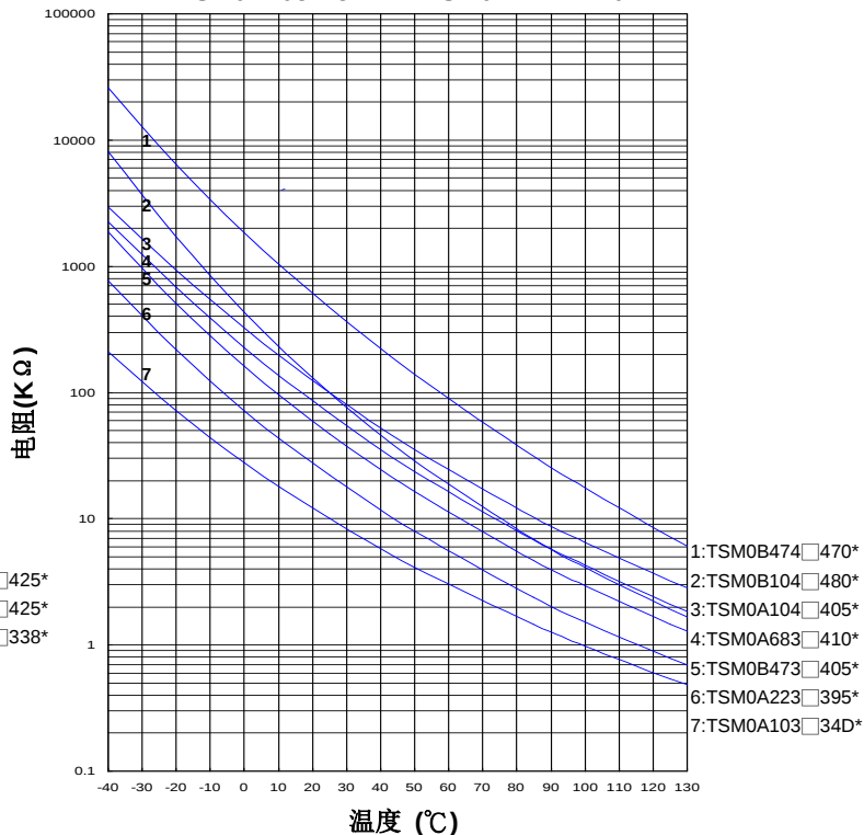
TSM0A103□34D* ~ TSM0B474□470*
